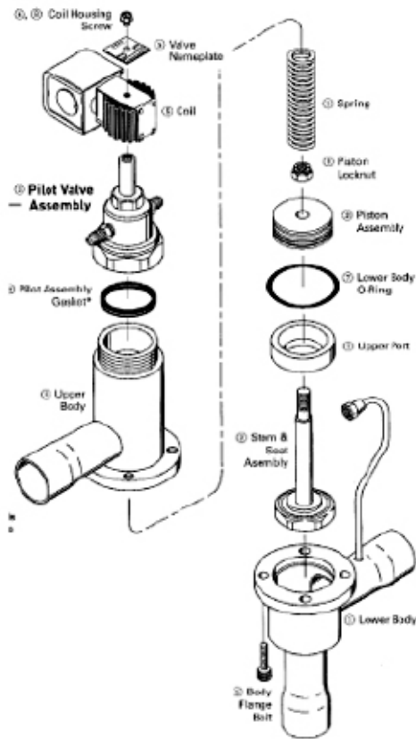
Heat Reclaim Valve
