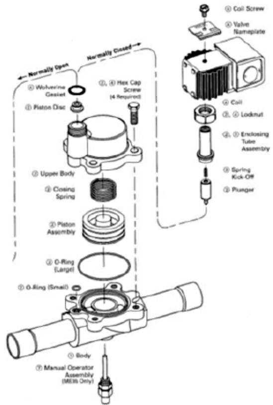
Solenoid Valve
